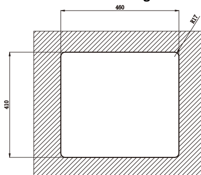
Cut-out Dimension Diagram
