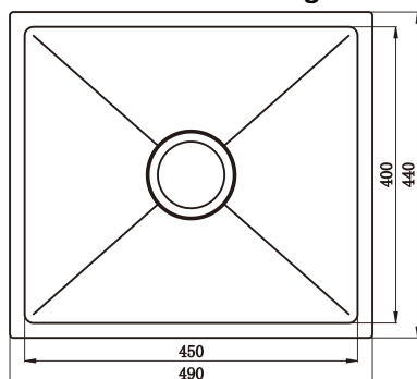
Overall Dimension Diagram
